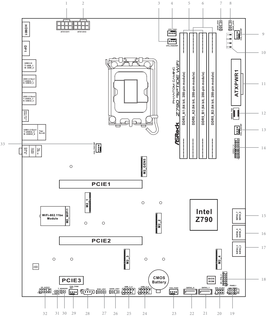
Top Side View
